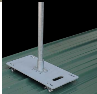
1 10' Schedule 40 Rail Part # 427302
